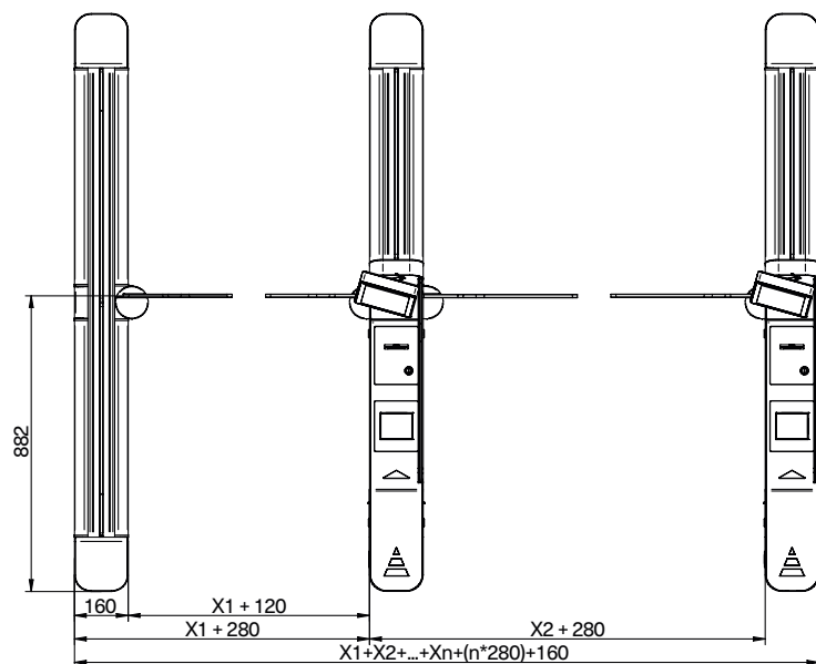
mPass (2-line configuration) – top view
